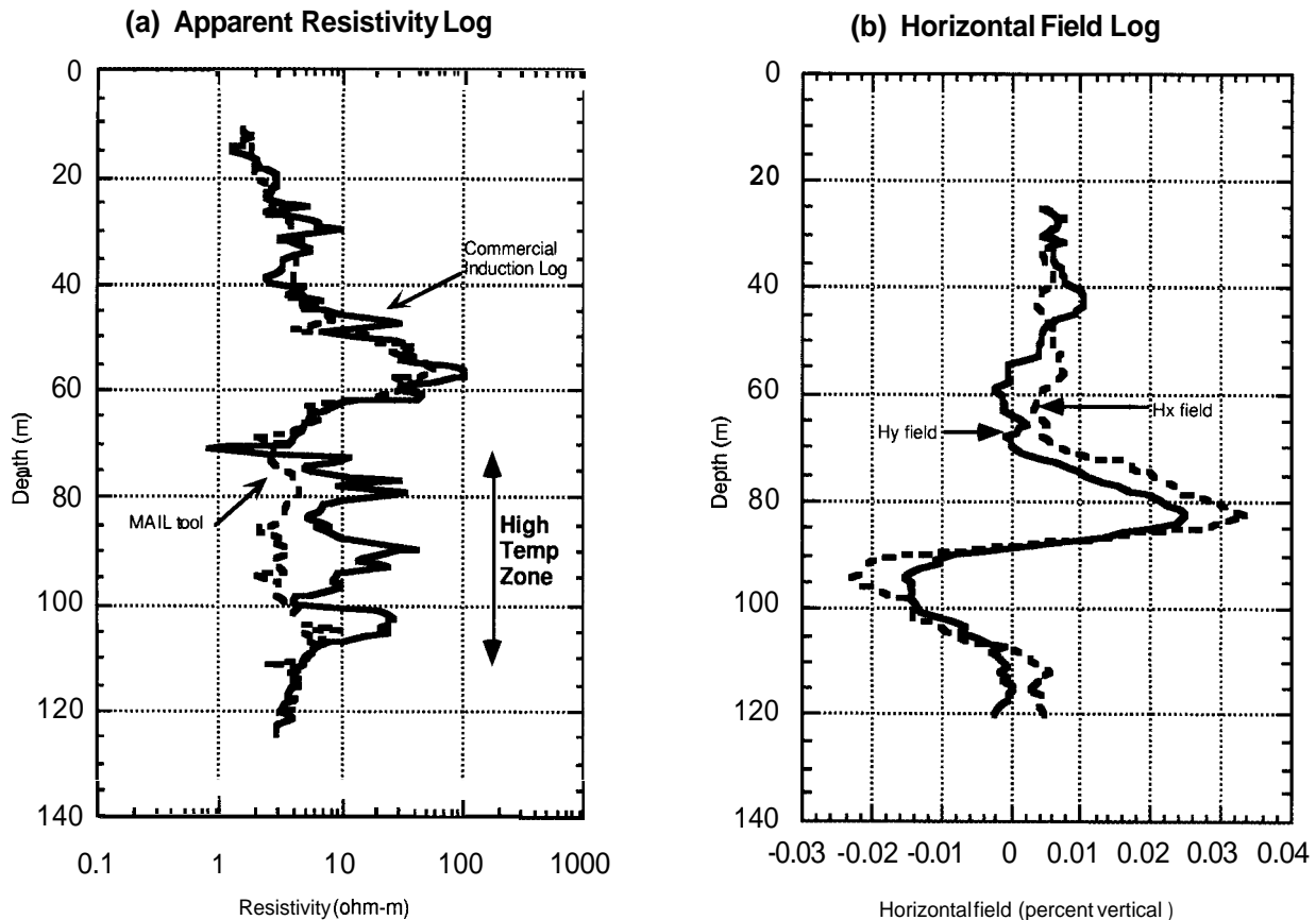
Fig. 2. (a) Comparison of apparent resistivity logs measured with the MAIL tool and conventional induction logging data in the same borehole. Note: the MAIL data was collected after steam injection. (b) Horizontal magnetic fields from the MAIL in the same borehole.
