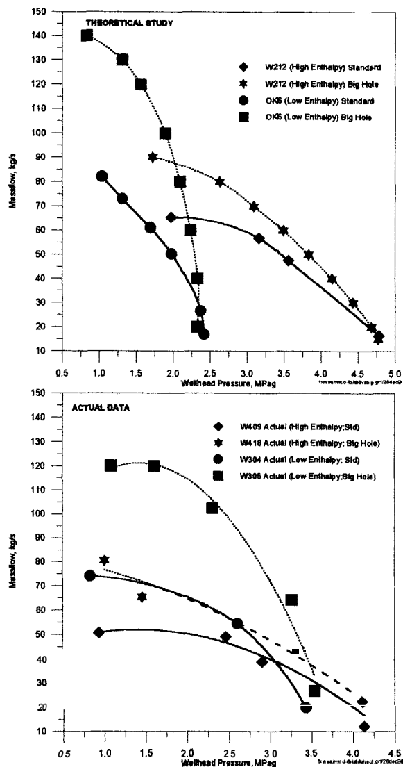
Figure 2. Effect of casing size on well output for low- and highenthalpy feed for theoretical and actual wells (from Sta. Ana 1989 and 1996).
