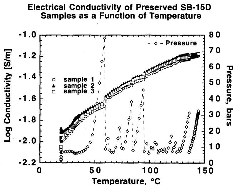
Fig. 4. Plot of log conductivity (S/m) as a function of temperature for three samples. Confining pressure is shown on the second y-axis. Pressure was manually controlled and needed to be reduced as temperature increased. A strong temperature dependence which correlates with the temperature dependence of pore fluid conductivity is observed. Increasing pressure decreases total electrical conductivity but is a secondary effect (see text).
