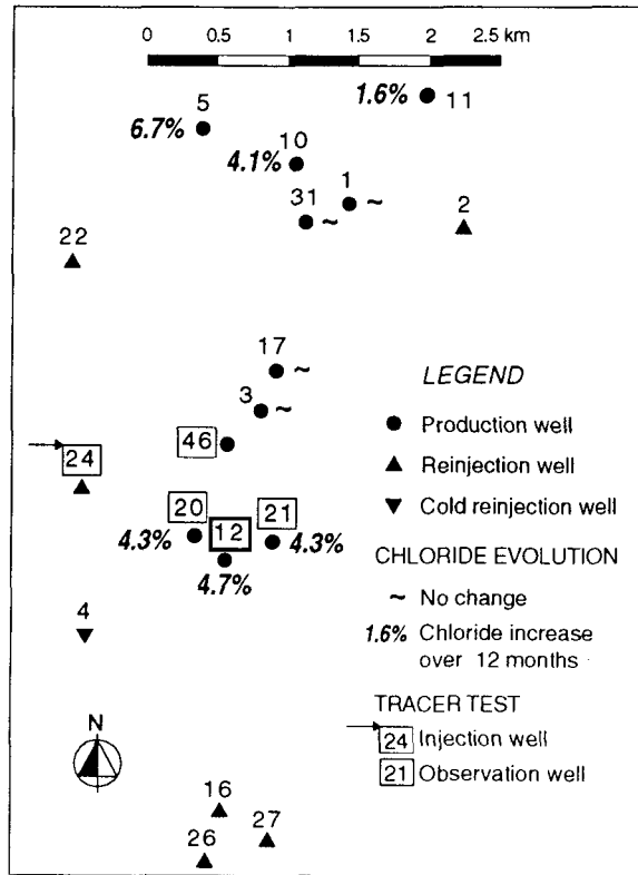
Figure 3. Evolution of Chloride Content and Tracer Test Arrangement
