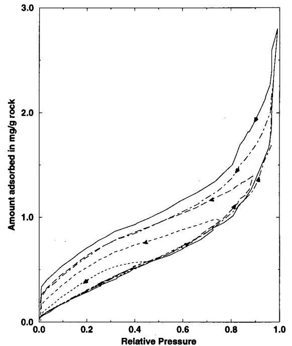
Figure 7: Scanning curves obtained for a sample from NEGU-17 at 120 °C.
