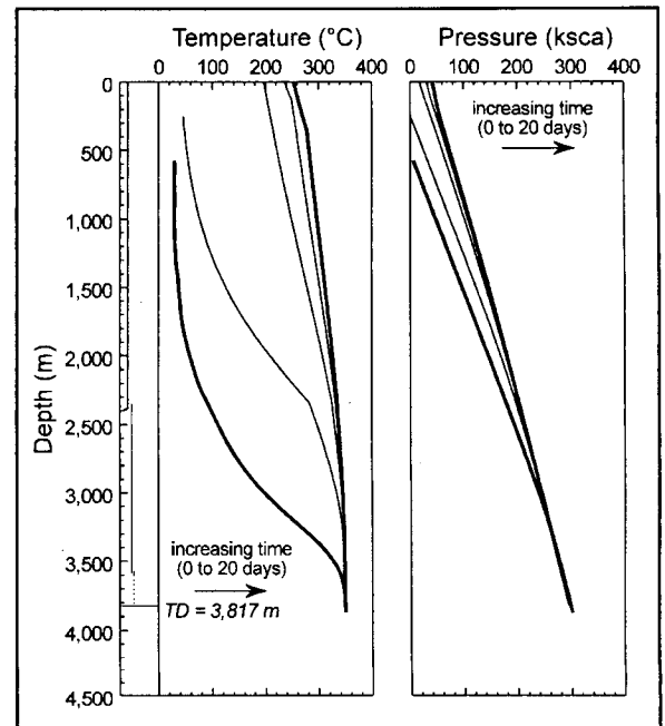
Figure 9: Wellbore simulation results; flow from well = 300 liters/minute
