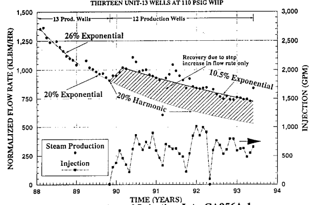
FIG. 3: Effect of Injection Into CA956A-1 on Some Surrounding Prod. Wells.
