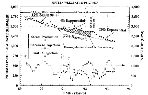
FIG. 5: Effect of Injection in Barrows-1 on Surrounding Wells
