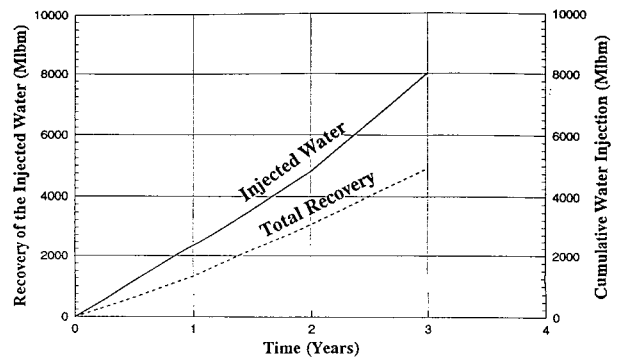
FIG. 3: Effect of Injection Into CA956A-1 on Some Surrounding Prod. Wells.
