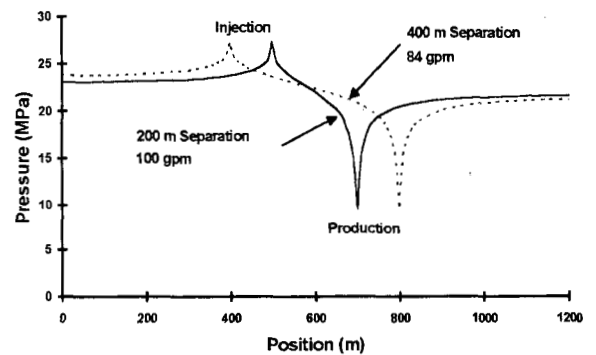
Figure 5. Pressure Profiles for Two Wellbore Spacings.
