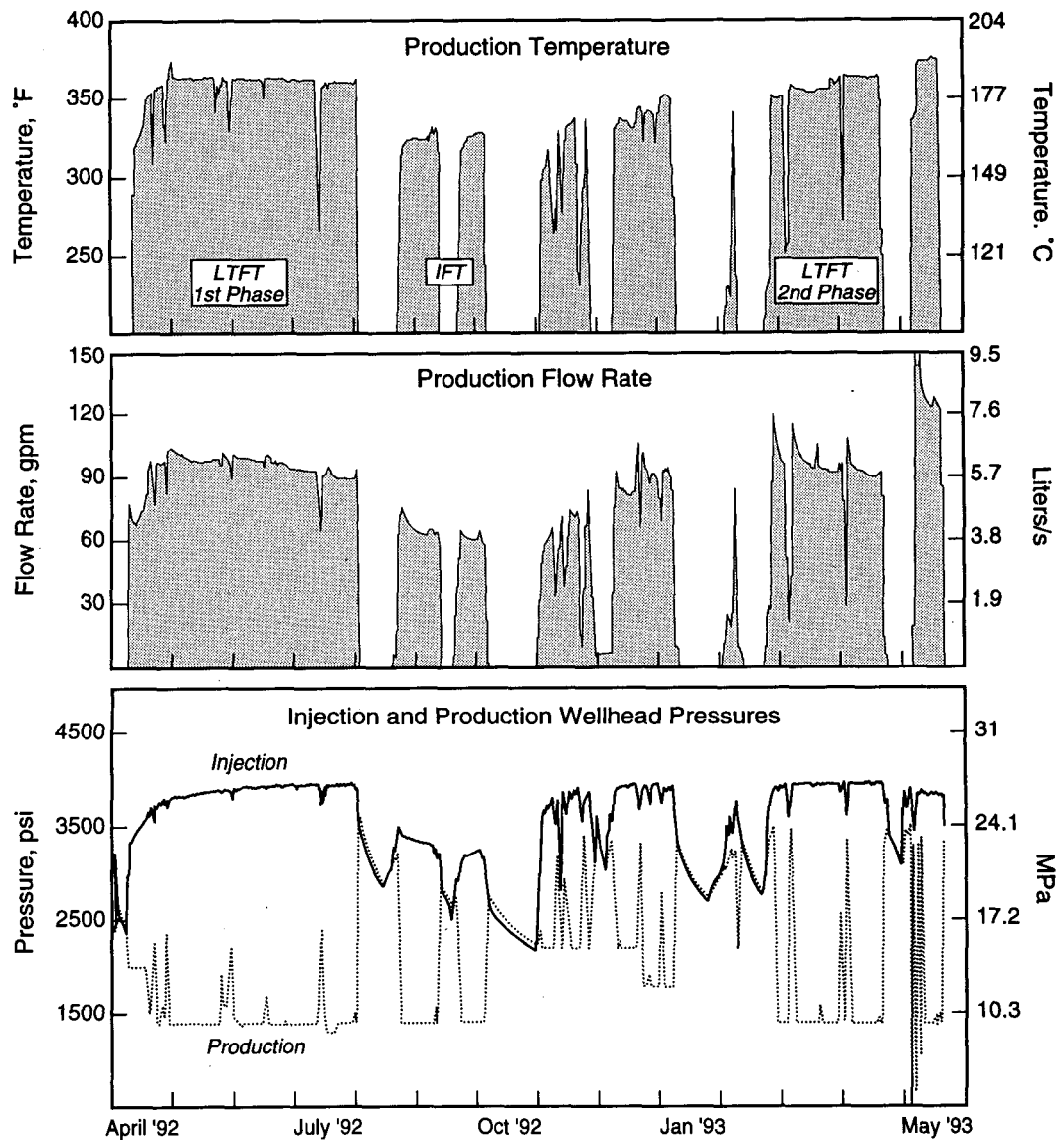
Figure 1. Fenton Hill Reservoir Operating Conditions from April 1992 to May 1993.
