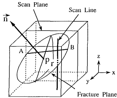
Figure 5 Concept of three dimensional fracture network model.
