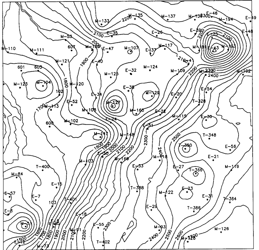
Figure 9. Map of the top of the producing intervals (depths in meters) of Cerro Prieto wells in the beta reservoir (Ricardo Márquez, CFE Cerro Prieto; personal commun., 1991).
