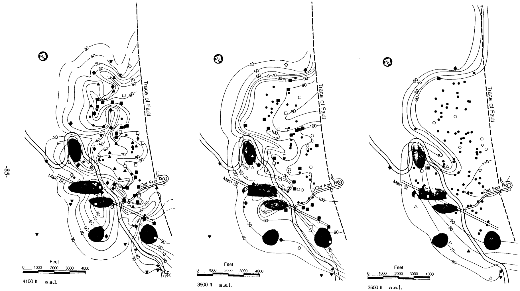
Figure 7. Temperature contour maps drawn at 4100 ft, 3900 ft and 3600 ft.
