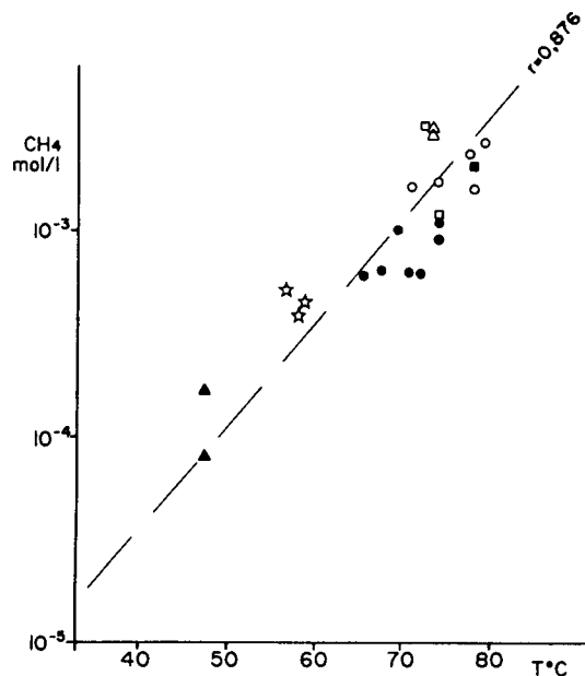
Figure 2 : Correlation between \text{CH}_4 content and downhole temperature.
