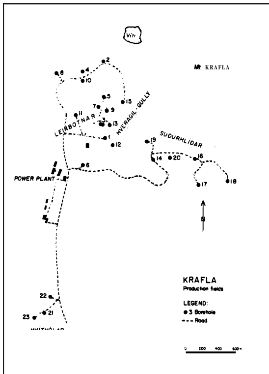
Figure 1. The production fields for the Krafla geothermal power plant.
