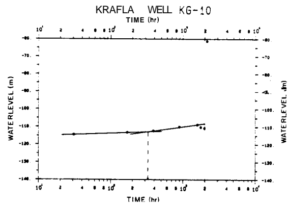
Figure 2. Waterlevel data from well 10 in Leirbotn.
