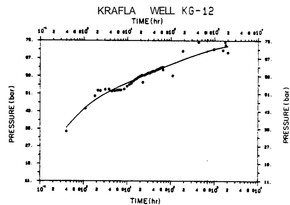
Figure 3. Pressure response of well 12 in Leirbotn.
