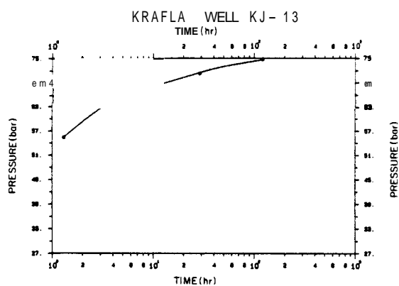
Figure 4. Pressure data from well 13 in Leirbotnar.
