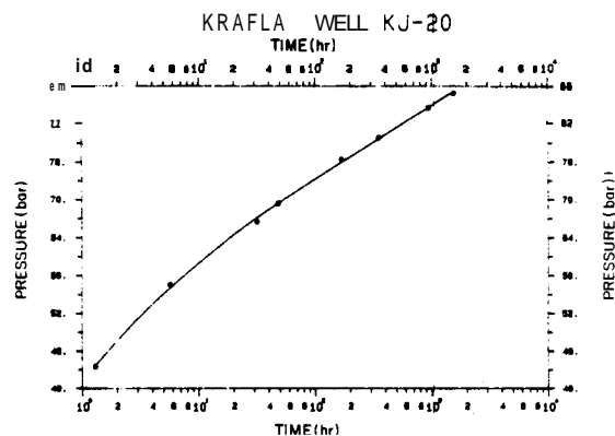
Figure 8. Pressure response of well 20 in Sudurhlidar.
