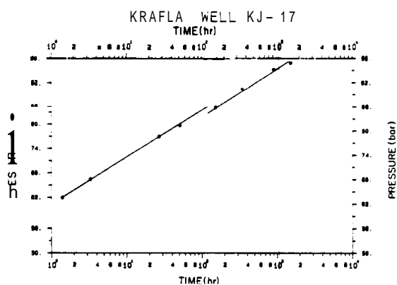
Figure 7. Pressure response of well 17 in Sudurhlidar.
