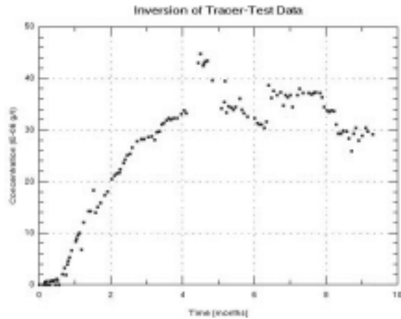
Figure 4. Raw tracer data plotted versus time. No background and decay correction is needed for the data because the tracer has zero concentration initially in the reservoir and does not degrade at temperatures below 300°C.
