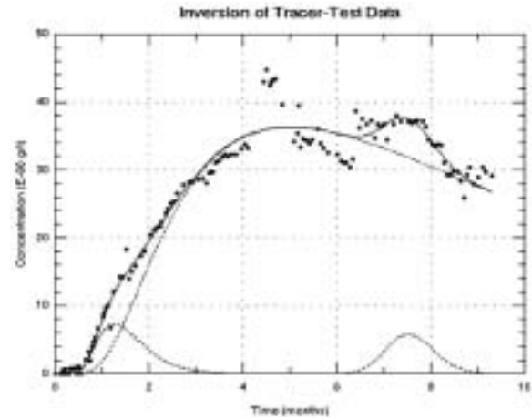
Figure 5. Result of simple one-dimensional channel tracer transport model superimposed on actual tracer data. The coefficient of determination of the model and actual data is 97%. Three tracer pulses may be responsible for the tracer curve behavior in well SK2D.
