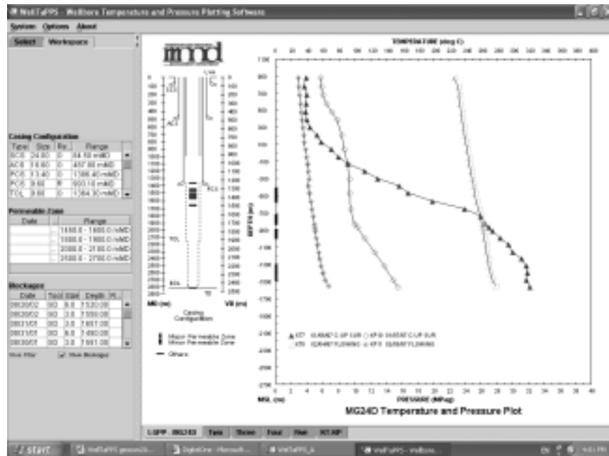
Figure 4. The temperature and pressure profiles of a production well and the wells basic information such as permeable zones, blockage surveys and casing configuration are tabulated by WellTaPPS.
