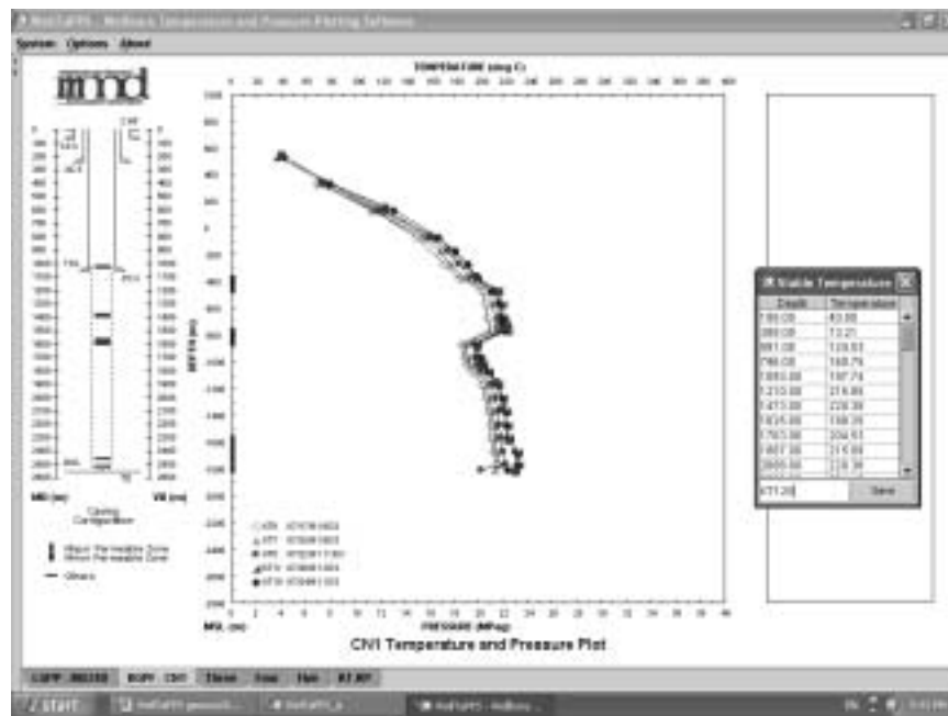
Figure 7. From a series of temperature surveys stable temperatures are generated by just right-clicking inside the plotting area. Stable temperature data points are connected by dashed lines to distinguish them from measured data.
