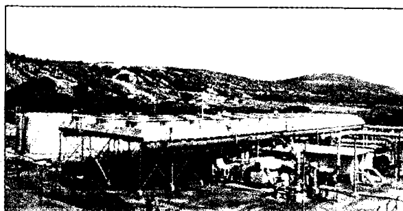
Figure 10. Sao Miguel No. 1 5 MW OEC Two Phase Geothermal Power Plant.
