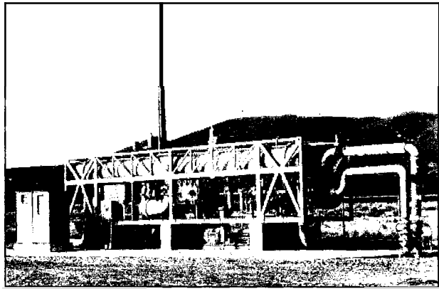
Figure 5. Enterprise 750 kW Unit No. 1.
