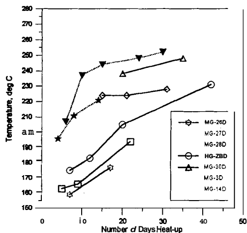
Fig. 2. Heat-up trend of Mahanagdong wells at -600 mRSL
