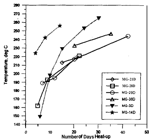
Fig. 3. Heat-up trend of Mahanagdong wells at -1000 mRSL
